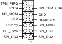
SPI_TPM_J1
